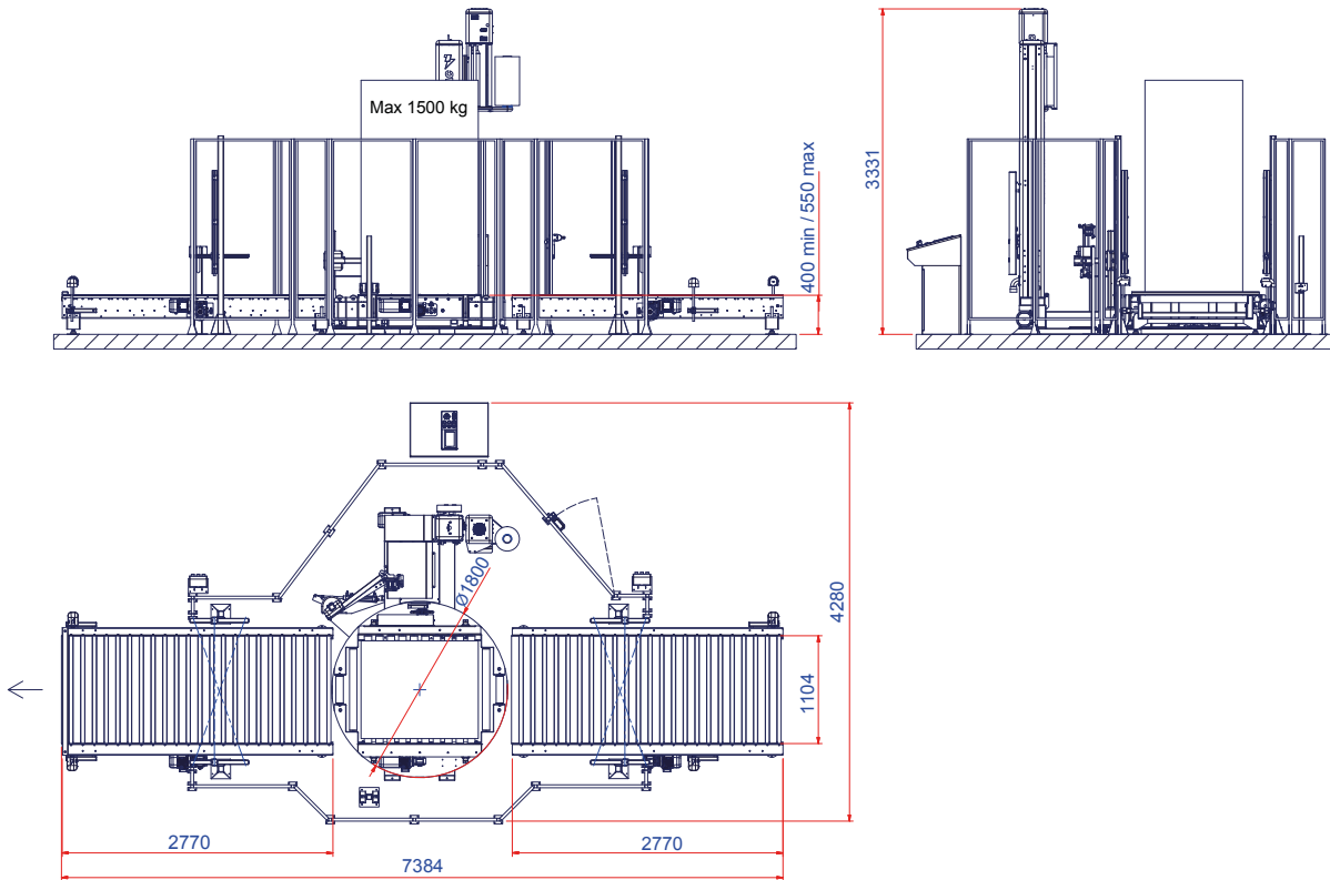
LAYOUT TECHNOPLAT 2000 PVS [mm]
